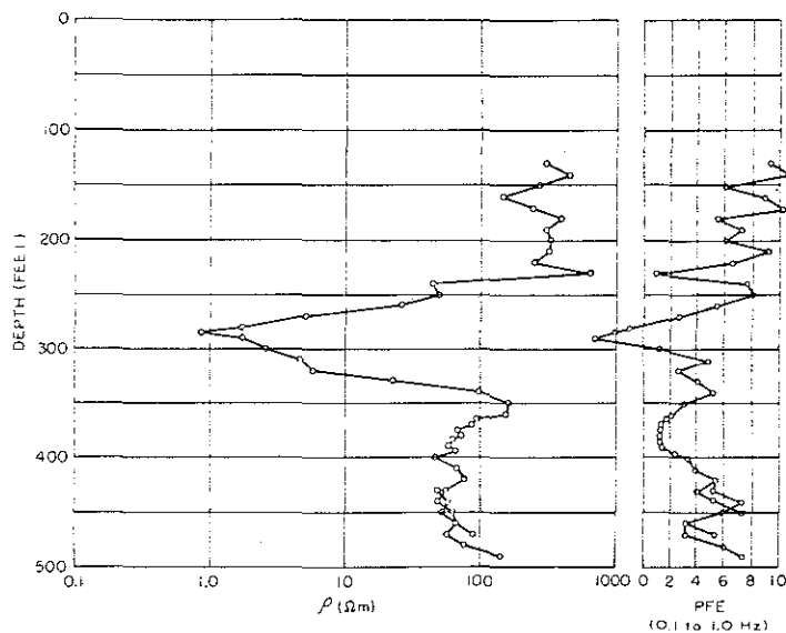
FIGURE 11. IP/RESISTIVITY LOG. DDH 22-3
