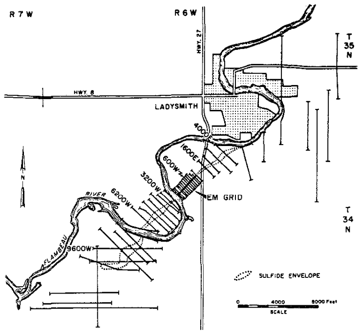
FIGURE 13. INDUCED POLARIZATION PLAN MAP
