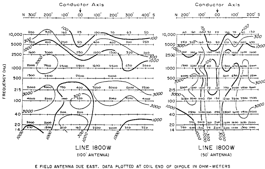
FIGURE 10. MAGNETOTELLURIC PROFILES
