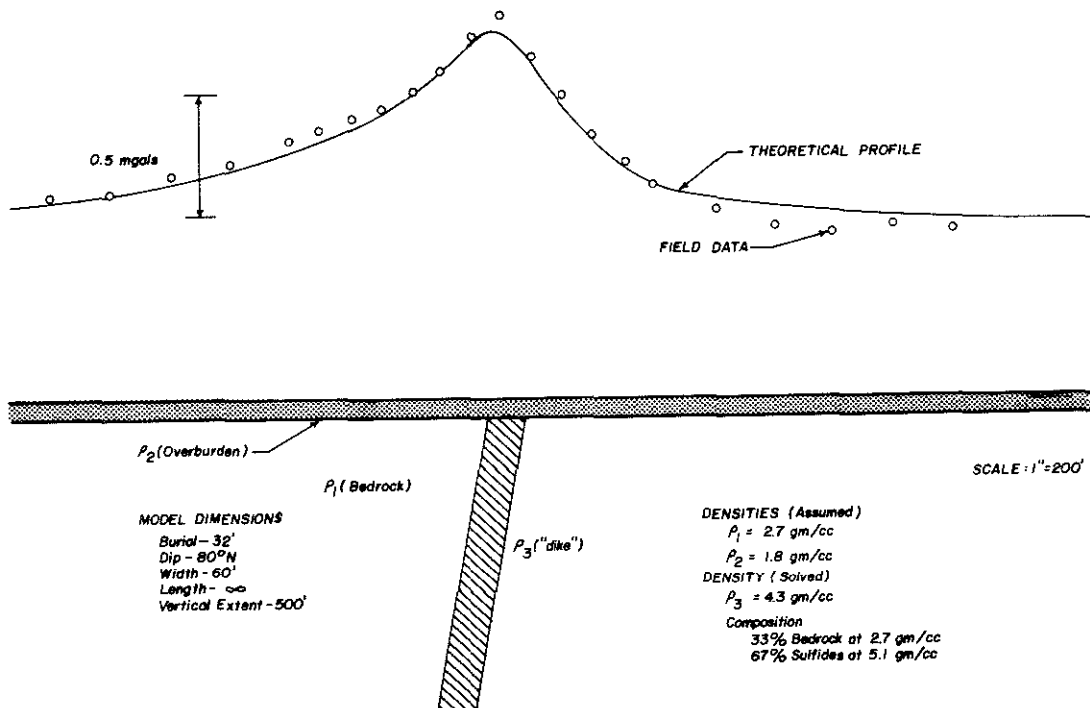
FIGURE 6. GEOPHYSICAL MODEL OF TARGET.
