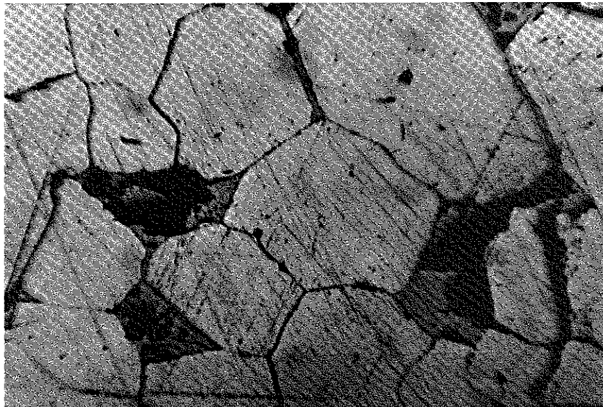
Figure 9. Photomicrograph of massive sulfide mineralization. Typical section of massive sulfide mineralization showing polygonal-shaped pyrite grains and interstitial chalcopyrite (light gray); pyrite grain shapes are probably the result of recrystallization. Pyrite grains about 0.5 mm. Reflected light.
