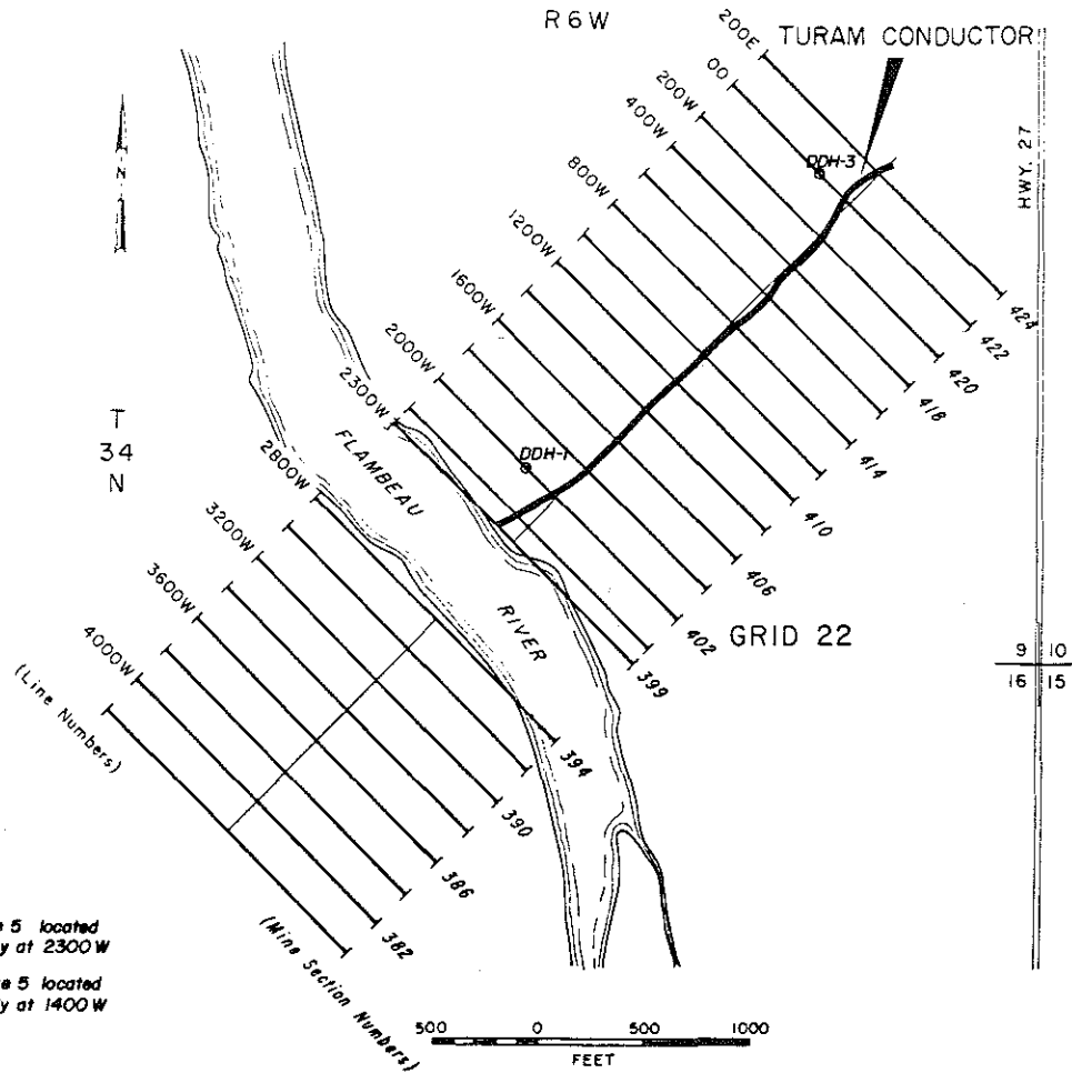
FIGURE 7. CONDUCTOR PLAN MAP
